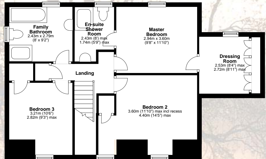
First Floor Approx. 59.1 sq. metres (635.9 sq. feet)
